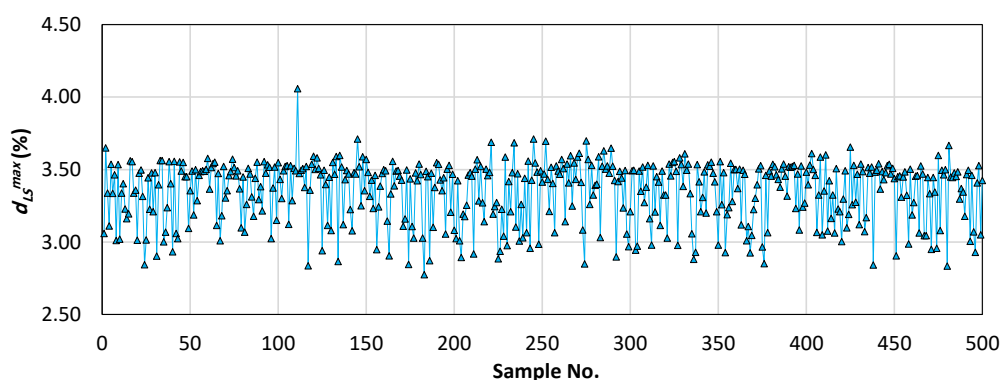
Figure 16: Maximum inter-story drift ratios at the LS level for the 12-story frame
