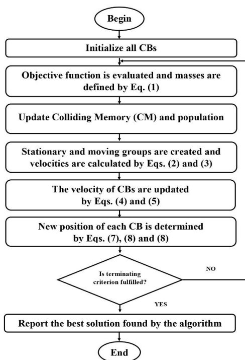
Figure 2. Flowchart of the ECBO algorithm [28]
