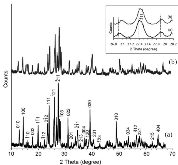
Fig. 1. XRD patterns of the prepared \text{Ag}_6\text{Mo}_{10}\text{O}_{33} (a) and Ni-substituted \text{Ag}_6\text{Mo}_{10}\text{O}_{33} (b).
