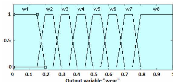
Fig. 22. Drill wears membership function
