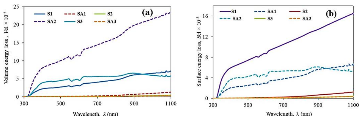
Fig. 19. a) Volume energy loss and b) surface energy loss for the prepared films
