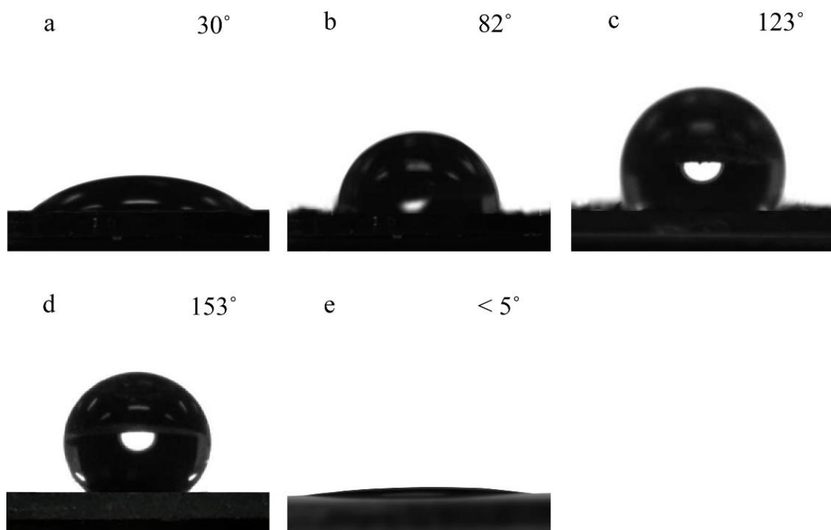
Fig. 3. Image of \mu L 5 drops of water on the surface of the coating a) Uncoated glass substrate, b) HMDS-modified particle coating, c) PDMS coating, d) TSP3 coating e) TSP3 sample after treating in 450^\circ for 2 hours
