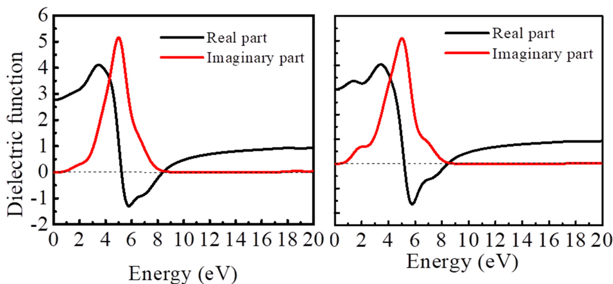
(a) \text{Sr}_{0.875}\text{Cr}_{0.125}\text{TiO}_3
