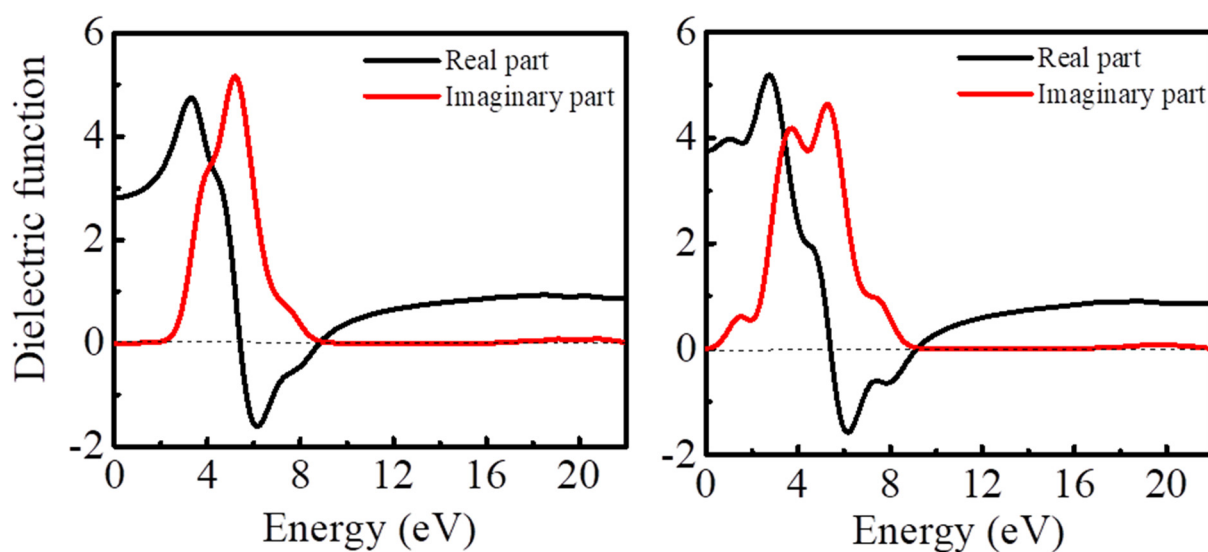
(a) \text{SrTi}_{0.875}\text{Cr}_{0.125}\text{O}_3
