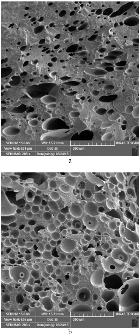
Fig. 2. SEM picture of nanocomposite foam samples, a) PA-6 containing 1 wt% MWCNT and b) PA-6 containing 1.5 wt% MWCNT
