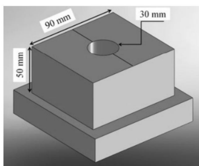
Fig. 1. Schematic drawing of casting mould.
