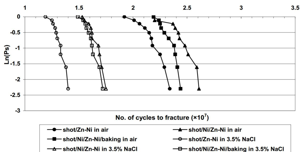
Fig. 6. Weibull diagram for number of cycles up to failure in fatigue corrosion test for assessment of environmental conditions effect
