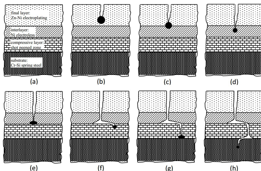
Fig. 7. Schematic of crack propagation in steel substrate in presence of a multilayer coating system containing Zn-Ni alloy and interlayer nickel. (This figure was developed based on research-work of Nascimento [15])
