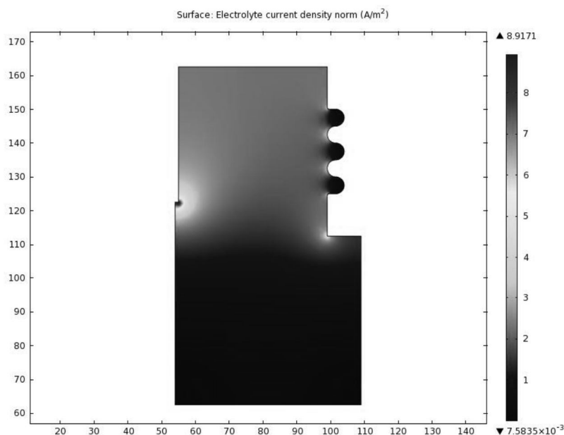
Fig. 5. Simulated Current Density in electrolyte
