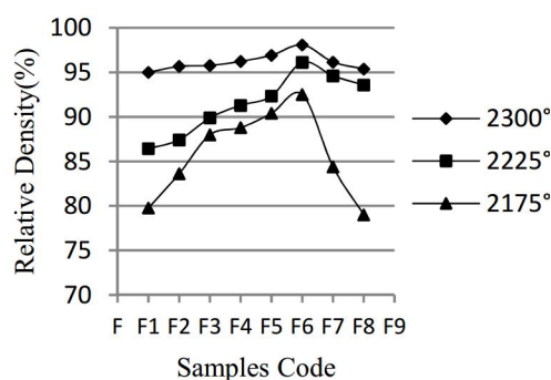
Fig. 4. Effect of Fe addition on relative density of F-Series samples sintered at various temperatures.
