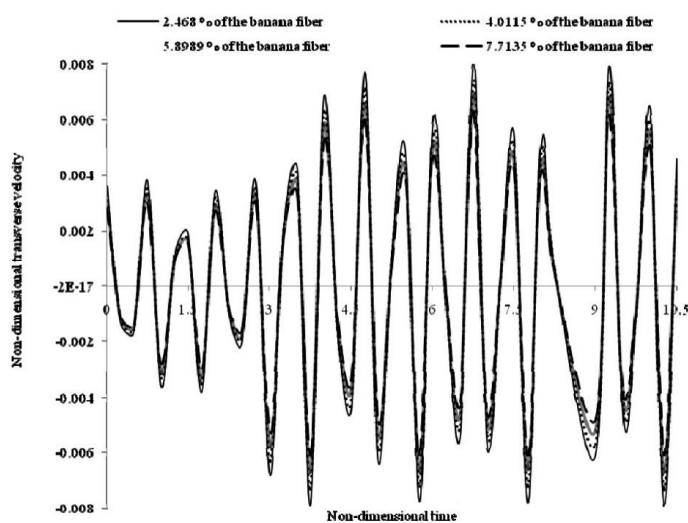
Fig. 20. Transverse-velocity of a simple supported randomly distributed short banana fiber reinforced composite plate at uniformly distributed load q = 10 \text{ N/m}^2 and different % of the fiber (rectangular pulse loading).
