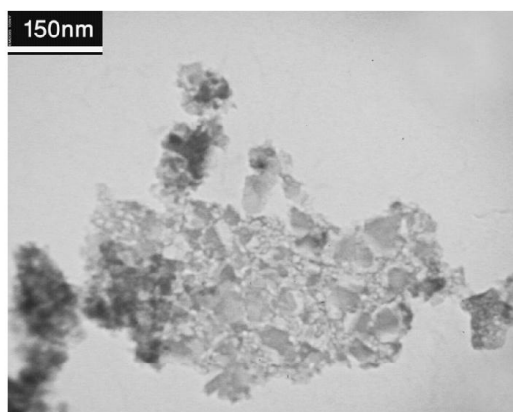
Fig. 2. Nano-size bioglass fabricated by sole-gel method.
