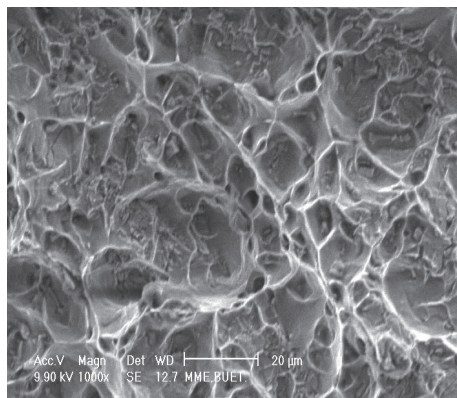
Fig. 8(d). Fractograph of plate 3 ( notch at HAZ)
