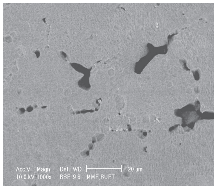
Fig. 7(a). BSE image of plate 1
