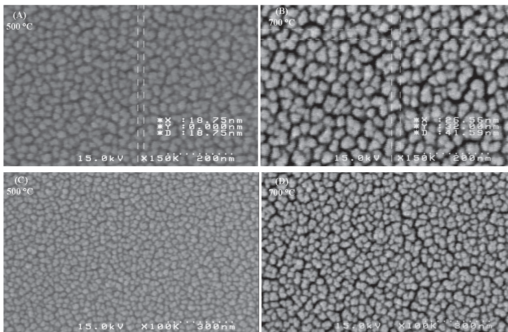
Fig. 3. FE-SEM micrograph of a \text{TiO}_2 - \text{SiO}_2 films annealed at (A,C) 500 °C, (B,D) 700 °C.
