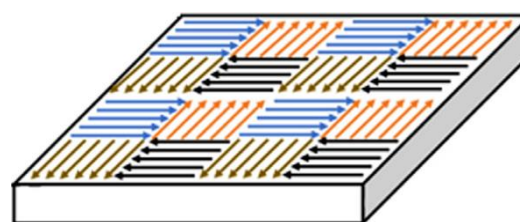
Fig. 10. Schematic of island scan strategy [148]
