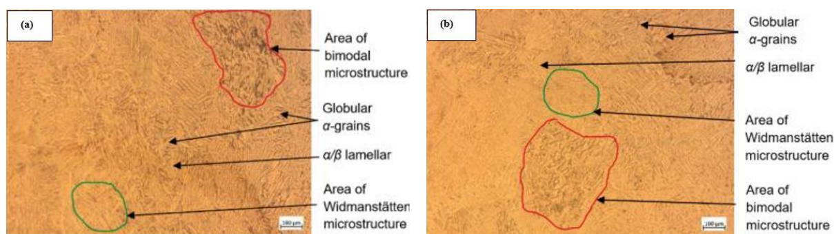
Fig. 13. Optical micrograph of a DMLS Ti6Al4V(ELI) sample that were stress relieved followed by high temperature annealed and tested at a temperature of 20°C (a) near the fracture surface (b) 15 mm away from the fracture surface
