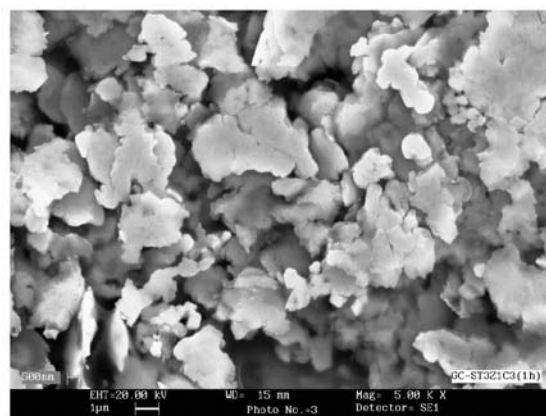
Fig. 6. SEM micrograph of ST 3 Z 1 (a) and ST 3 Z 1 C 3 (b) nucleated and crystallized at T n and T p .
