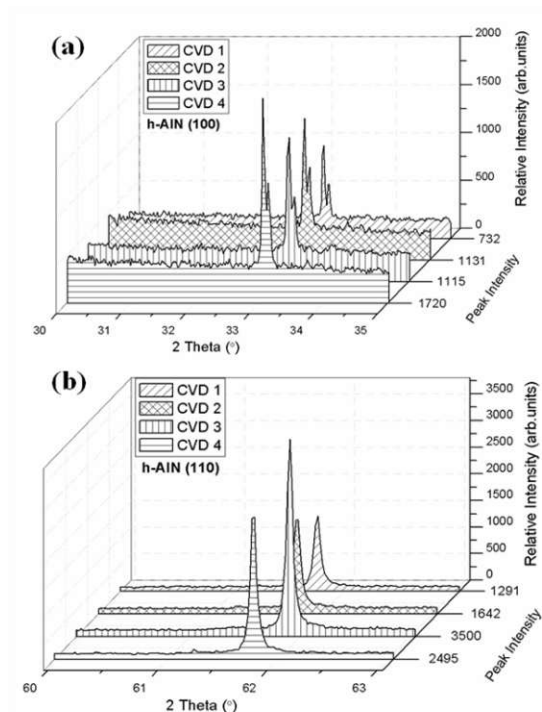
Fig. 3. Variation in XRD peak intensity of (a) (100), and (b) (110) oriented hexagonal AlN.
