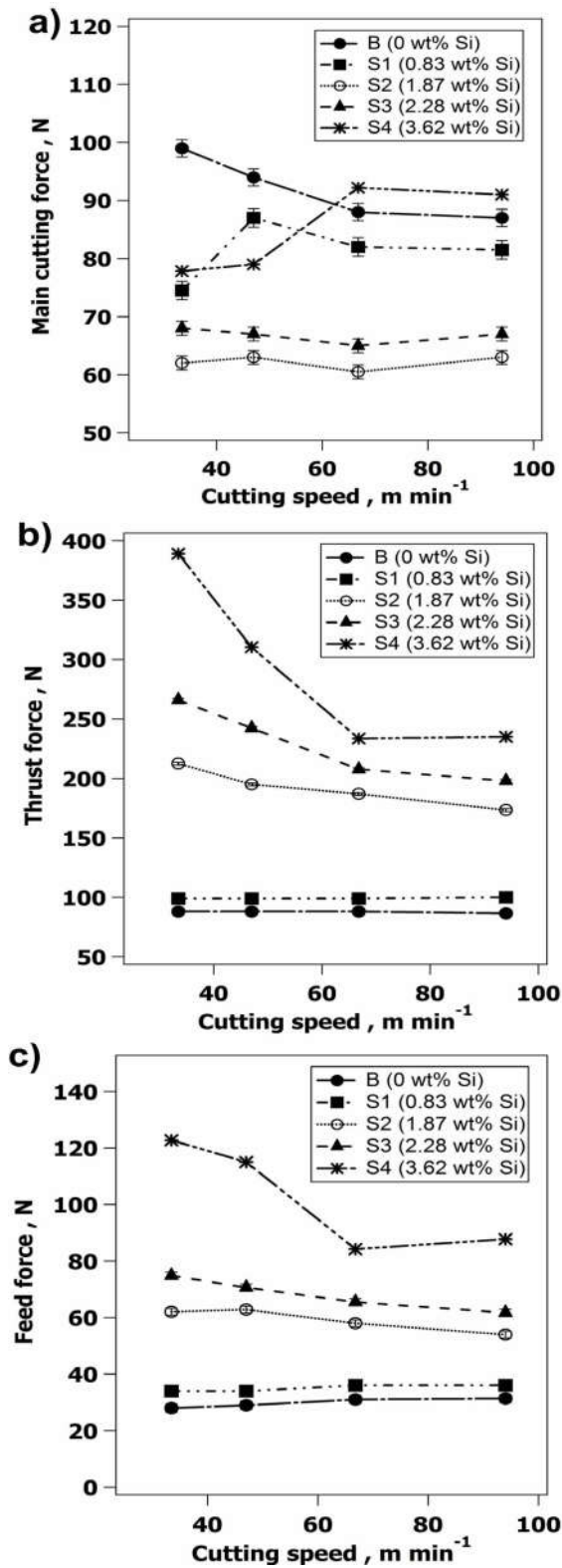
Fig. 12. Variation of cutting forces with cutting speed for Si-added samples
