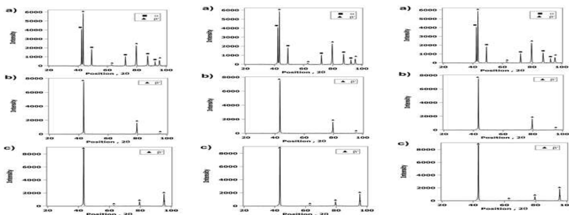
Fig. 4. XRD patterns obtained from samples (a) A1, (b) A2 and (c) A3
