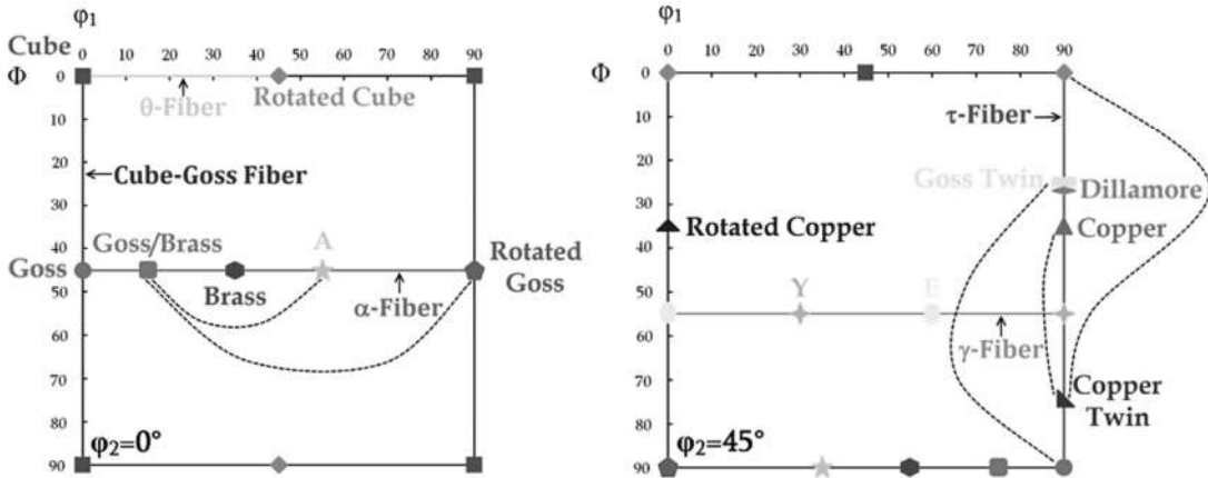
Fig. 7. Schematic illustration of the important texture components in FCC materials. The dashed lines depict twin relationships [22].
